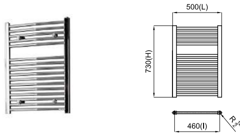
500x730 mm
