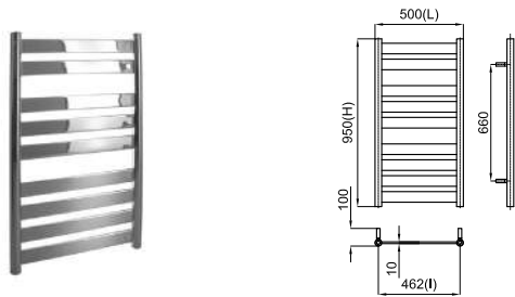
500x950 mm
