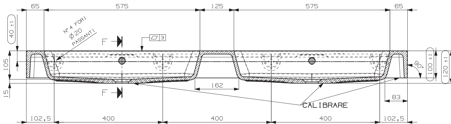
SECTION E-E SCALE 35:200
